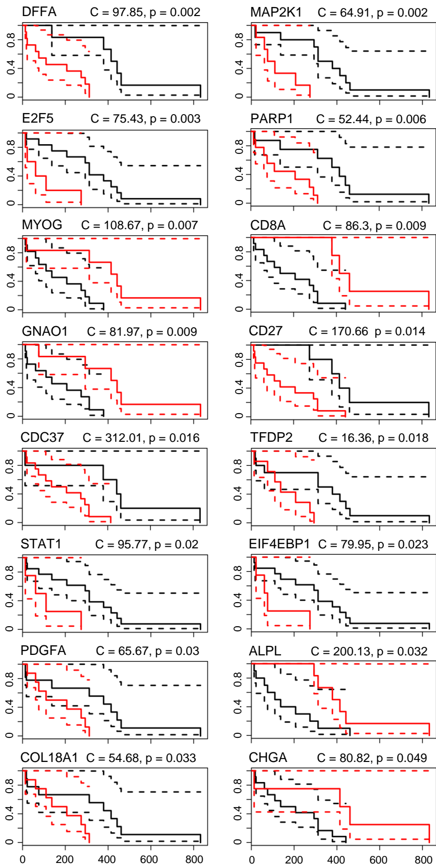
Sup. Image 2: Kaplan-Meier graphs of plasma levels of 16 proteins, associated with survival of GBM patients (C = critical value)
