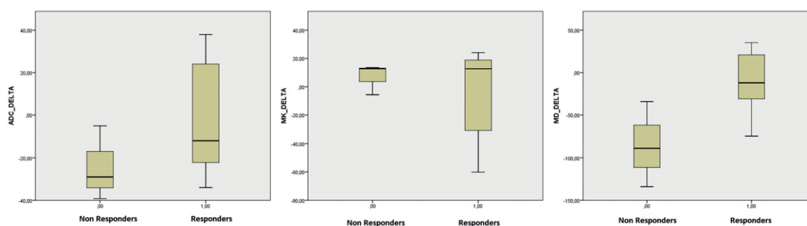
FIGURE 2. Boxplot of apparent diffusion coefficient (ADC) and diffusion kurtosis imaging (DKI) parameters percentage change values between responders and not responders.
