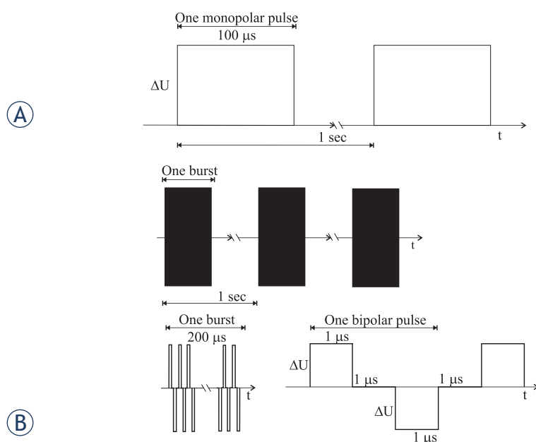
FIGURE 1. Scheme of the applied pulses. (A) 100 \mu s long monopolar pulses of amplitude \Delta U (80 V – 240 V in a step of 40 V) were applied with a repetition frequency of 1 Hz. (B) Short bipolar pulses (HF-EP). Above: 8 bursts were applied with a repetition frequency of 1 Hz. Down left: One burst was 200 \mu s long and consisted of 50 bipolar pulses. Below right: One bipolar pulse of amplitude \Delta U (100 V – 1000 V in a step of 100 V) consisted of 1 \mu s long positive pulse, 1 \mu s long negative pulse (both of voltage \Delta U ) with a 1 \mu s long delay between pulses.
