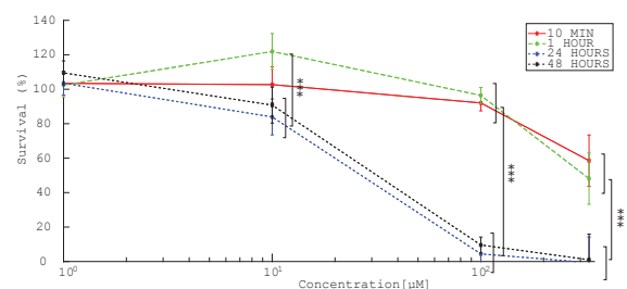
FIGURE 4. Cytotoxicity of cisplatin without electroporation at different concentrations and time of incubation. Each data point was repeated 4 times (mean ± standard deviation) and is normalized to the control sample in which cisplatin was substituted by 0.9% NaCl. A 2-way ANOVA was performed. 10 min or 1 h of incubation was different from 24 h or 48 h ( P < 0.001 ) while there was no difference between 10 min vs 1 h and 24 h vs 48 h. 330 µM cisplatin was more cytotoxic than other tested concentrations ( P < 0.001 ). There was no significant difference between 1 µM and 10 µM cisplatin; all other comparisons were significantly different ( P < 0.001 ).
