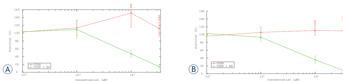
FIGURE 6. Cytotoxicity of cisplatin at different concentration of cisplatin (CDDP) and electroporation (EP) at a fixed value of electric field (A) 1.2 kV/cm, 8x100 μs long monopolar pulses, delivered at repetition frequency 1 Hz; (B) 3 kV/cm, 8 bursts of short bipolar pulses (HF-EP) of 1-1-1-1 μs, delivered at repetition frequency 1 Hz. Each data point was repeated 3-7 times (mean ± standard deviation). Each data was normalized to the control sample electroporated and with 0.9% NaCl instead of cisplatin. We performed a 2-way ANOVA. For both types of pulses, at 100 μM and 330 μM the CDDP samples were significantly different from the CDDP+EP samples ( P < 0.001 ).
