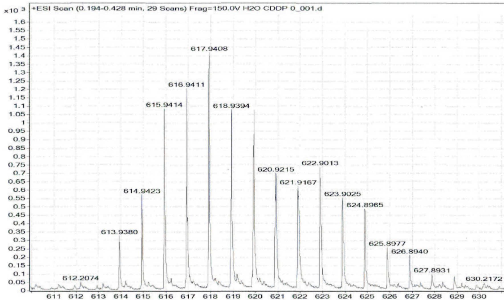
SUPPLEMENTAL FIGURE S8. Zoom-scan high-resolution mass spectrometry (HRMS) spectrum ( m/z 610–630) of cisplatin in water without application of electric pulses with observed peak for [2M+NH_4]^+ ( m/z 617.9408).
