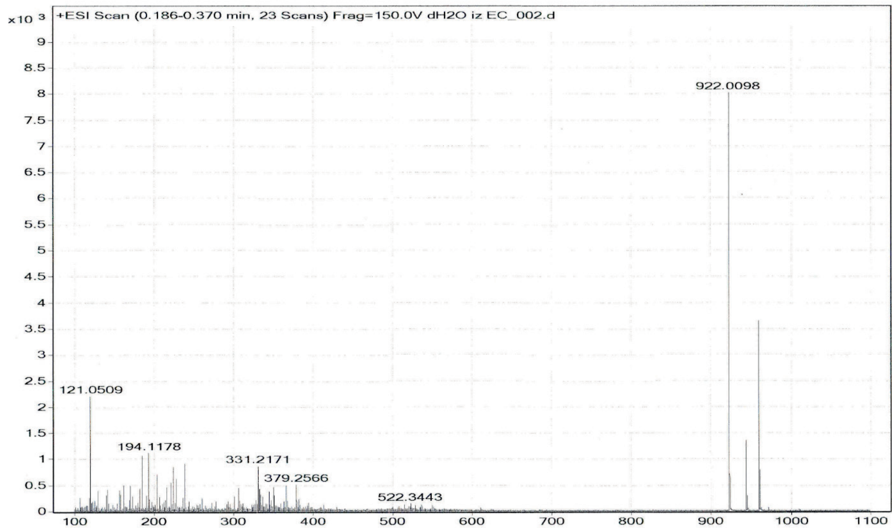
SUPPLEMENTAL FIGURE S19. Full-scan high-resolution mass spectrometry (HRMS) spectrum of water from electroporation cuvette without application of electric pulses.
