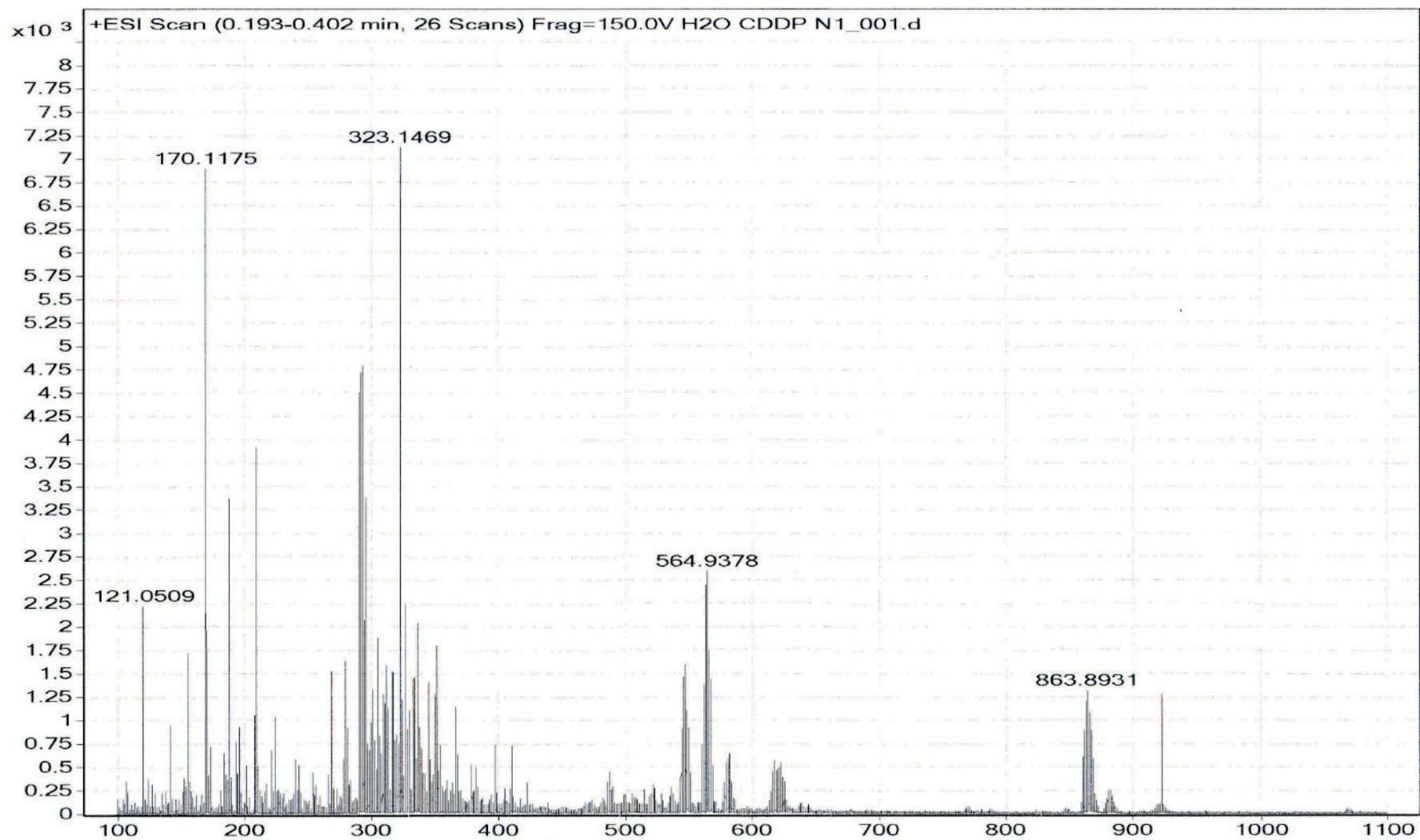
SUPPLEMENTAL FIGURE S11. Full-scan high-resolution mass spectrometry (HRMS) spectrum of cisplatin in water after nanosecond pulses application.
